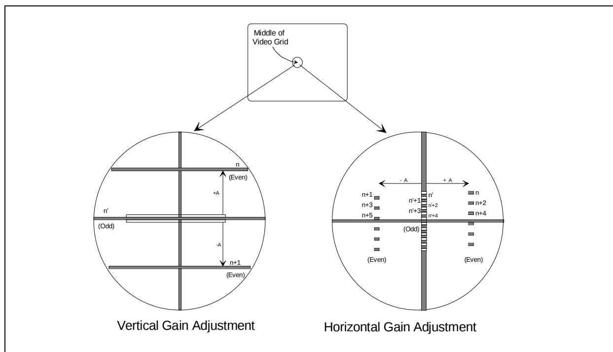
Figure 27. Gain Cursors
