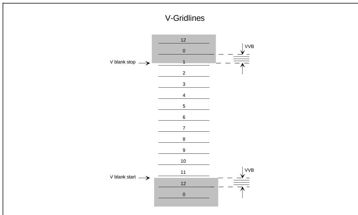
Figure 25. Vertical Blanking
