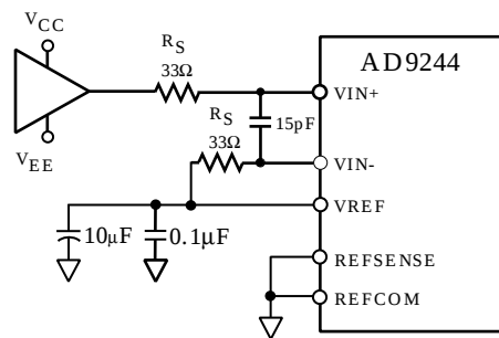
Figure 3. Resistors Isolating SHA Input from Op Amp
