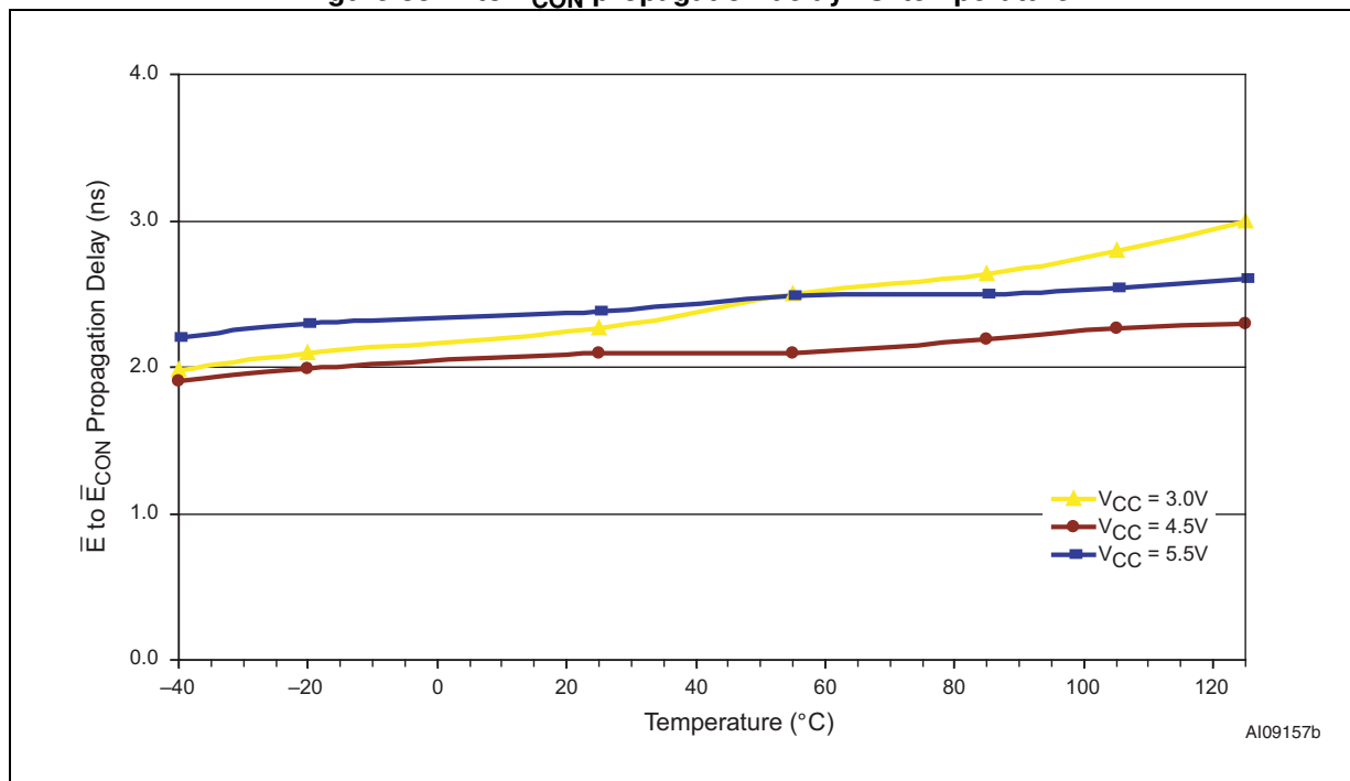
Figure 38. \bar{E} to \bar{E}_{\text{CON}} propagation delay vs. temperature
