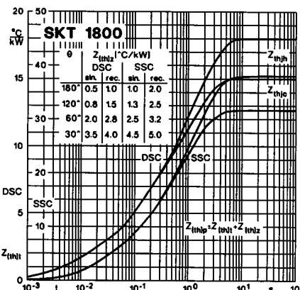
Fig. 4 a Transient thermal impedance vs. time
