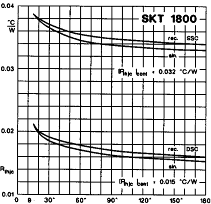
Fig. 5 a Thermal resistance vs. conduction angle
