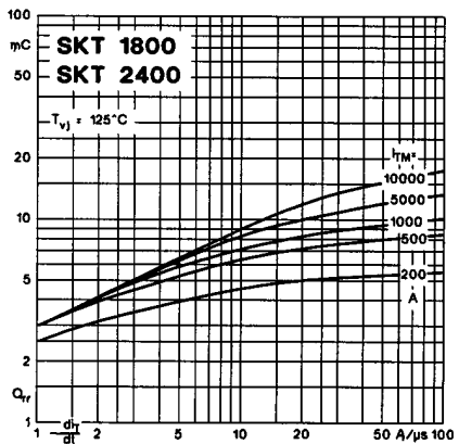
Fig. 3 Recovered charge vs. current decrease
