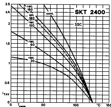
Fig. 2 d Rated on-state current vs. case temperature
