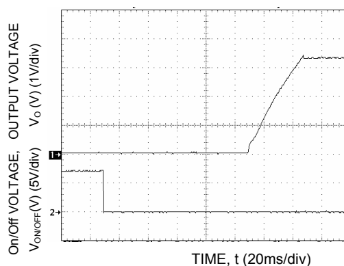
Figure 60. Typical Start-Up Using Remote On/Off, negative logic version shown.
