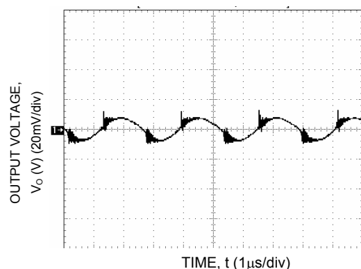
Figure 50. Typical Output Ripple and Noise.
