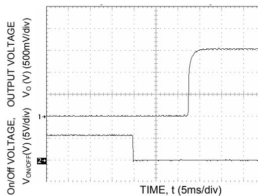
Figure 36. Typical Start-Up Using Remote On/Off, negative logic version shown.
