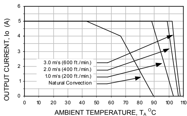
Figure 58. Derating Output Current versus Local Ambient Temperature and Airflow.
