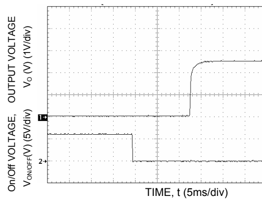
Figure 18. Typical Start-Up Using Remote On/Off, negative logic version shown.
