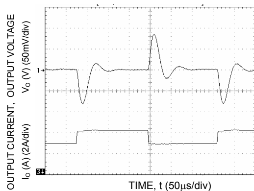
Figure 33. Transient Response to Dynamic Load Change from 50% to 75% to 50% of full load.
