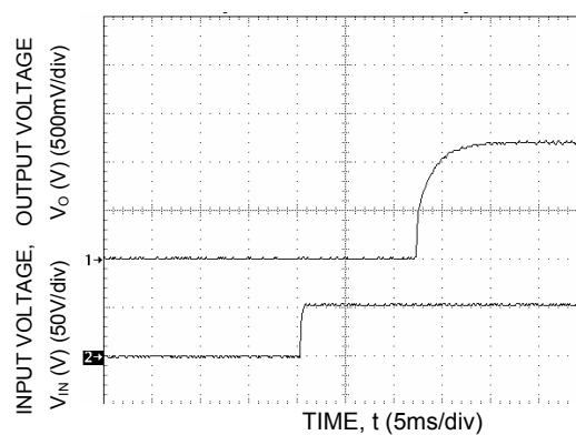
Figure 41. Typical Start-Up with application of Vin.
