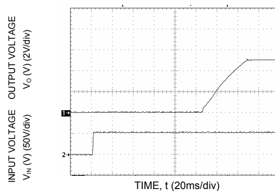
Figure 5. Typical Start-Up with application of V_{in} .
