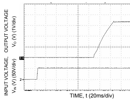
Figure 11. Typical Start-Up with application of V_{in} .
