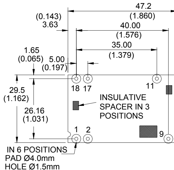
Through-Hole Pad Layout – Component side view
