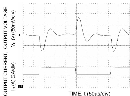
Figure 9. Transient Response to Dynamic Load Change from 50% to 75% to 50% of full load.
