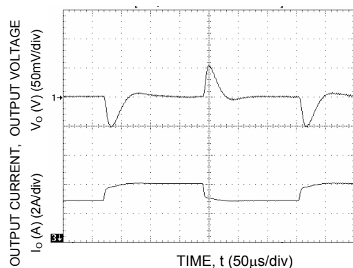
Figure 45. Transient Response to Dynamic Load Change from 50% to 75% to 50% of full load.
