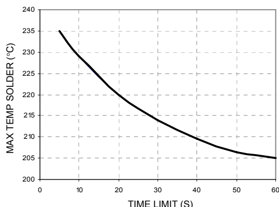
Figure 73. Time Limit Curve Above 205°C Reflow .
