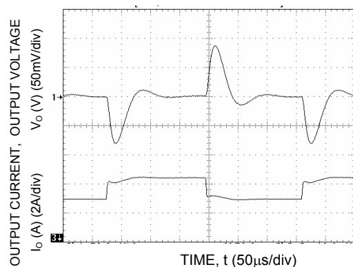
Figure 39. Transient Response to Dynamic Load Change from 50% to 75% to 50% of full load.
