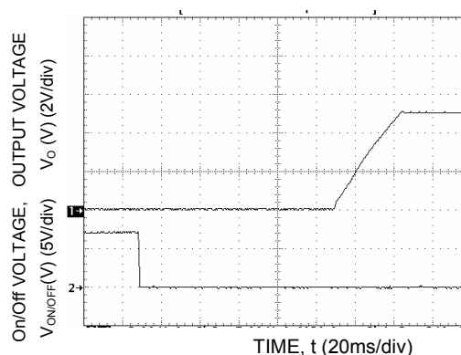
Figure 54. Typical Start-Up Using Remote On/Off, negative logic version shown.
