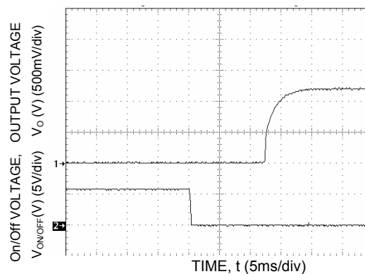
Figure 42. Typical Start-Up Using Remote On/Off, negative logic version shown.
