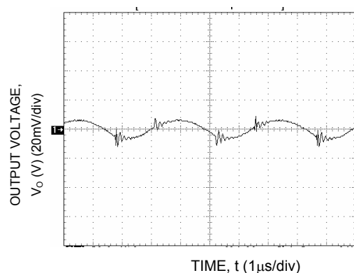
Figure 26. Typical Output Ripple and Noise.
