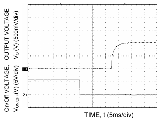
Figure 48. Typical Start-Up Using Remote On/Off, negative logic version shown.
