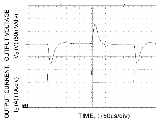
Figure 51. Transient Response to Dynamic Load Change from 50% to 75% to 50% of full load.
