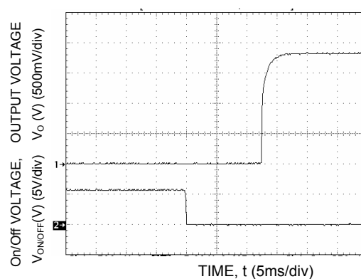
Figure 30. Typical Start-Up Using Remote On/Off, negative logic version shown.
