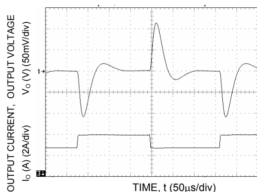
Figure 57. Transient Response to Dynamic Load Change from 50% to 75% to 50% of full load.
