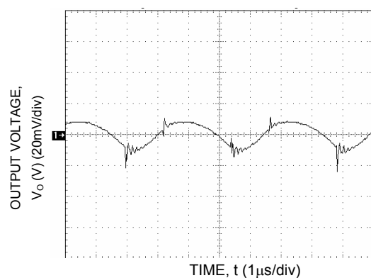
Figure 38. Typical Output Ripple and Noise.
