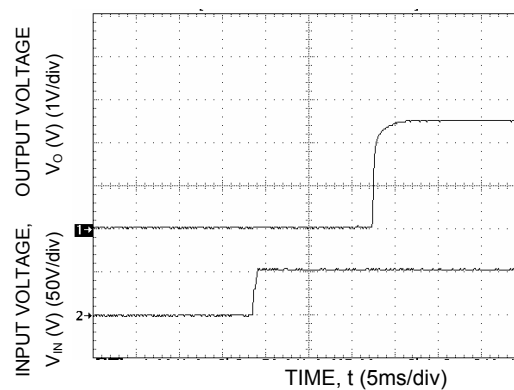
Figure 17. Typical Start-Up with application of V_{in} .
