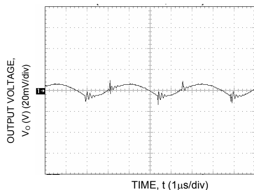
Figure 32. Typical Output Ripple and Noise.
