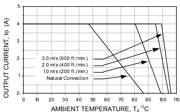
Figure 52. Derating Output Current versus Local Ambient Temperature and Airflow.
