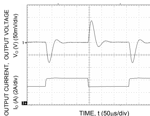
Figure 27. Transient Response to Dynamic Load Change from 50% to 75% to 50% of full load.
