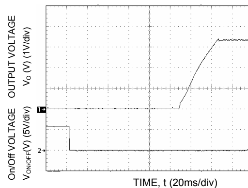
Figure 12. Typical Start-Up Using Remote On/Off, negative logic version shown.
