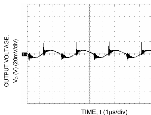
Figure 56. Typical Output Ripple and Noise.
