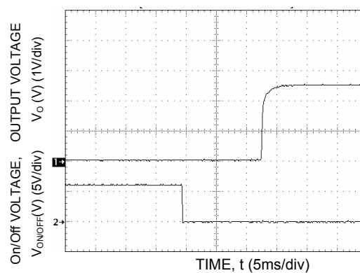
Figure 18. Typical Start-Up Using Remote On/Off, negative logic version shown.
