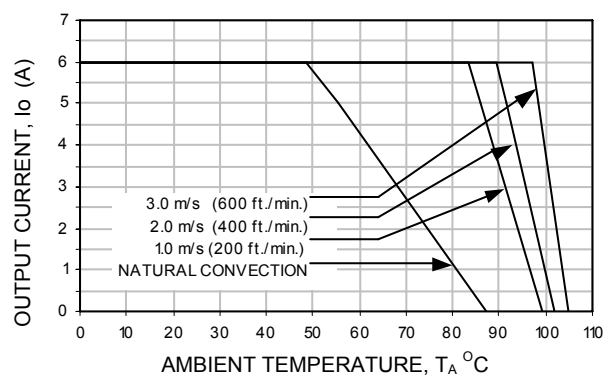
Figure 40. Derating Output Current versus Local Ambient Temperature and Airflow
