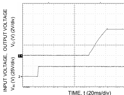
Figure 53. Typical Start-Up with application of V_{in} .
