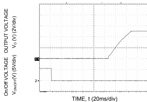
Figure 6. Typical Start-Up Using Remote On/Off, negative logic version shown.
