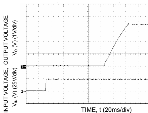
Figure 59. Typical Start-Up with application of V_{in} .
