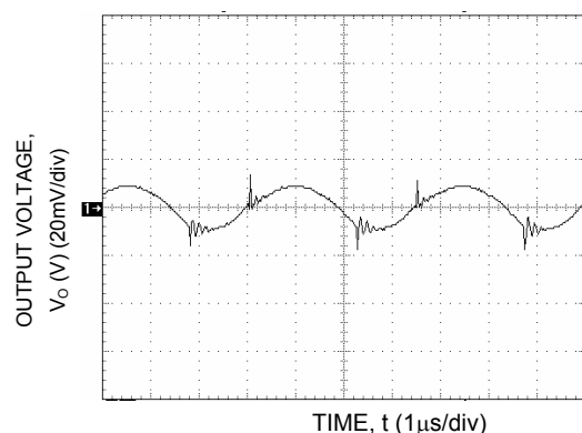
Figure 14. Typical Output Ripple and Noise.
