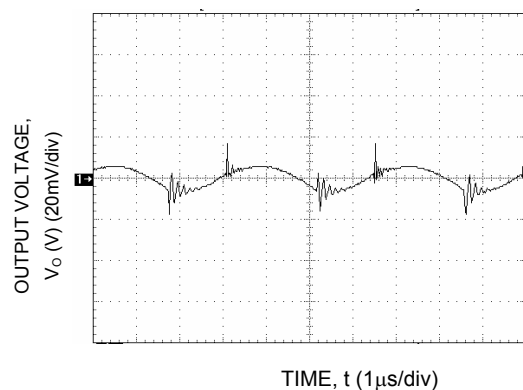
Figure 8. Typical Output Ripple and Noise.
