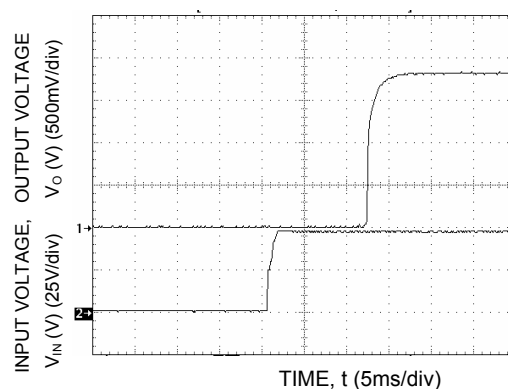
Figure 29. Typical Start-Up with application of V_{in} .
