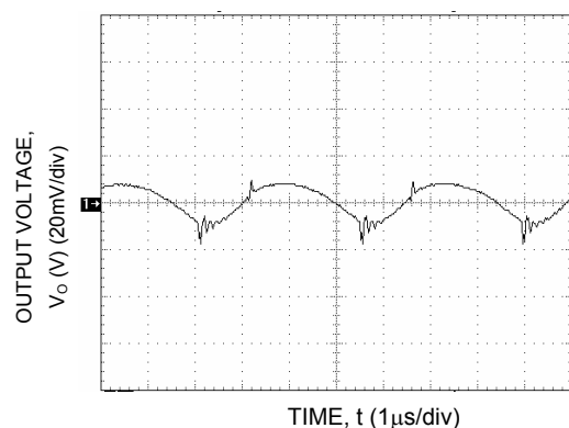
Figure 44. Typical Output Ripple and Noise.
