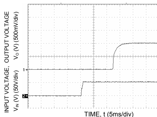
Figure 47. Typical Start-Up with application of V_{in} .
