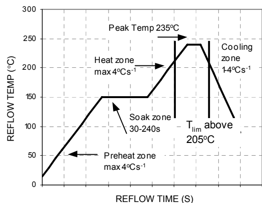
Figure 72. Recommended Reflow Profile
