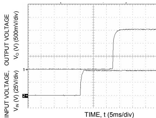
Figure 35. Typical Start-Up with application of V_{in} .
