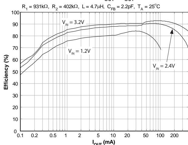
Efficiency vs. I_{OUT} ( V_{OUT} = 4.0V )
