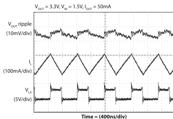
PWM Operation
