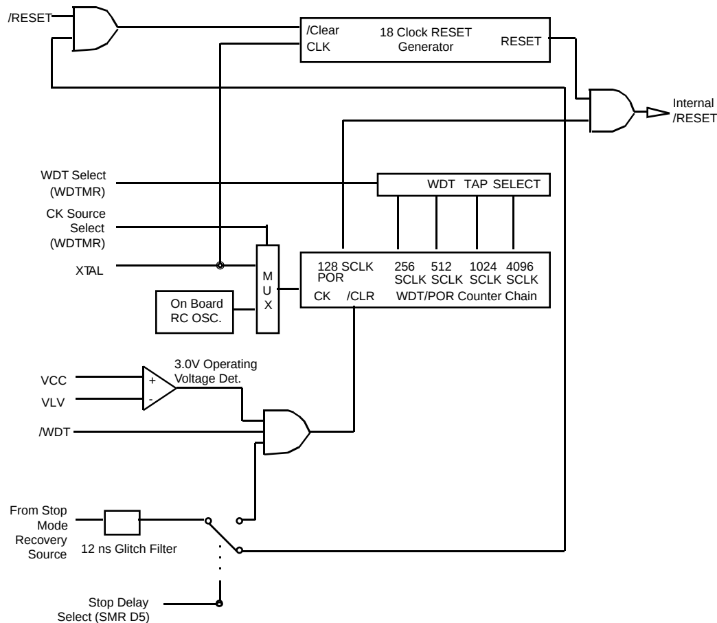
Figure 38. Resets and WDT
