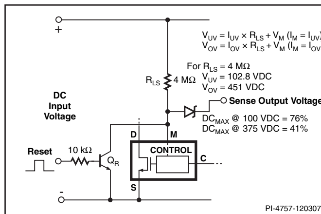
Figure 40. Line-Sensing for Undervoltage, Overvoltage, Line Feed-Forward and Latched Output Overvoltage Protection with Device Reset.
