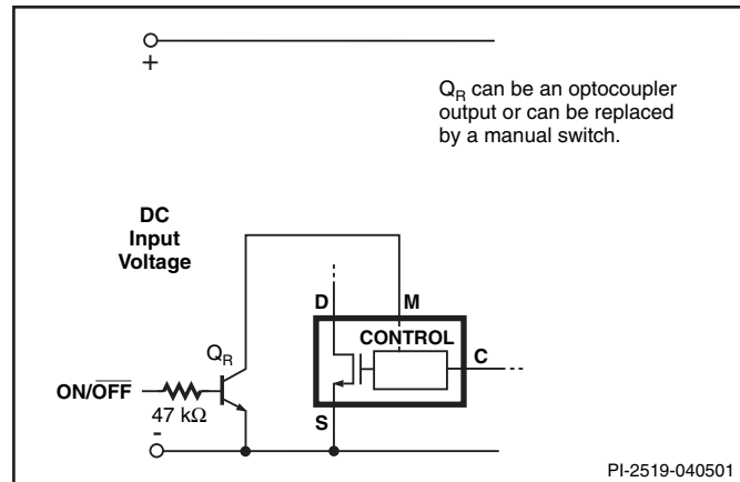
Figure 37. Active-on (Fail Safe) Remote ON/OFF.
