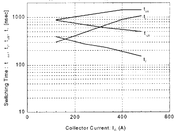
Switching Time vs. Collector Current V_{cc} = 600V, R_g = 2.7\Omega, V_{ge} = \pm 15V, T_J = 125^\circ\text{C}
