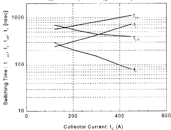
Switching Time vs. Collector Current V_{cc} = 600V, R_g = 2.7\Omega, V_{ge} = \pm 15V, T_J = 25^\circ\text{C}
