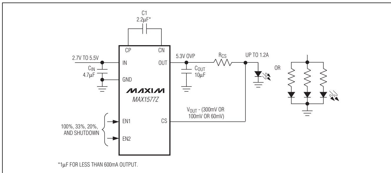
Figure 2. Current Regulation with the MAX1577Z
