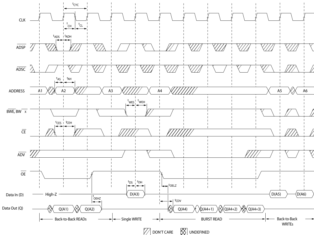
Figure 7. Read/Write Cycle Timing [27, 29, 30]
