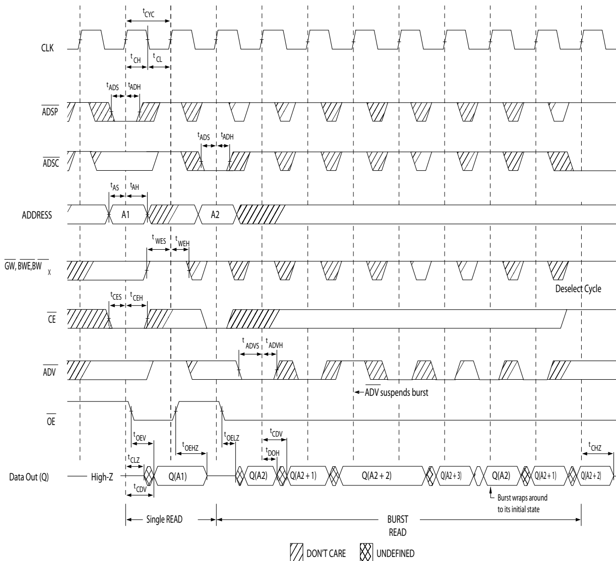
Figure 5. Read Cycle Timing [27]
