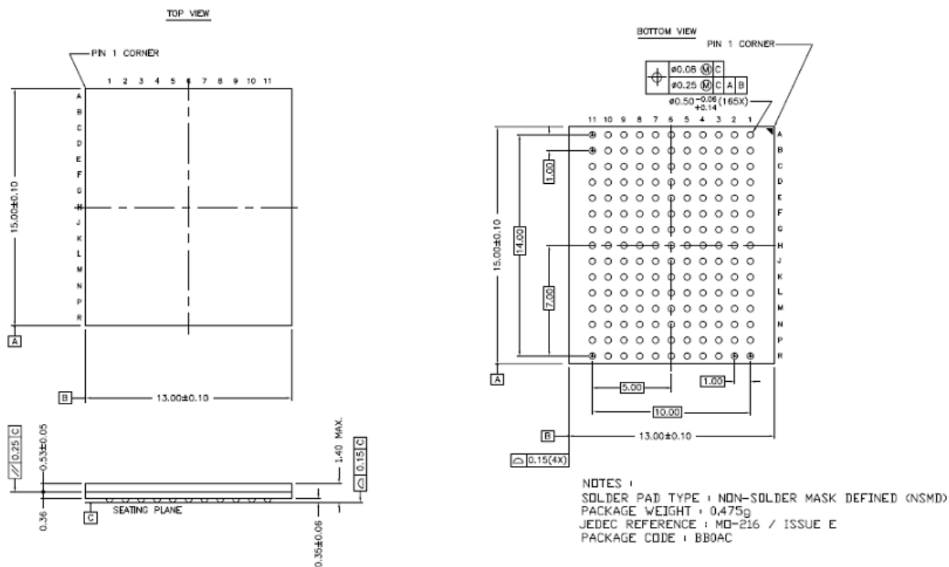
Figure 11. 165-Ball FBGA (13 x 15 x 1.4 mm) (51-85180)
