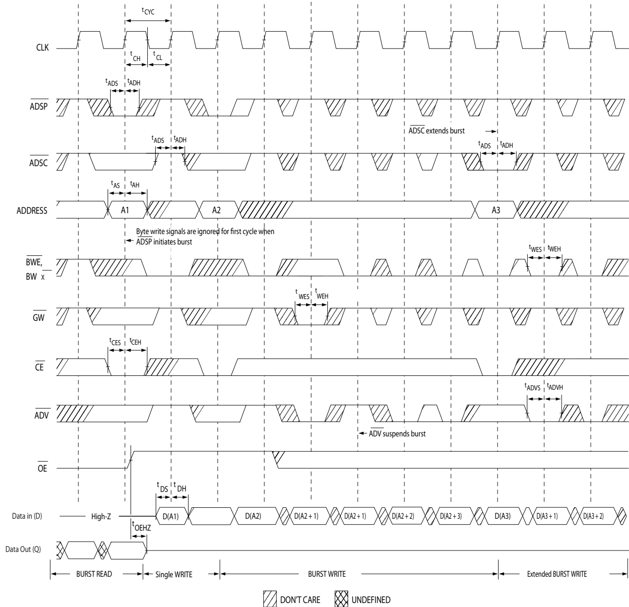
Figure 6. Write Cycle Timing [27, 28]
