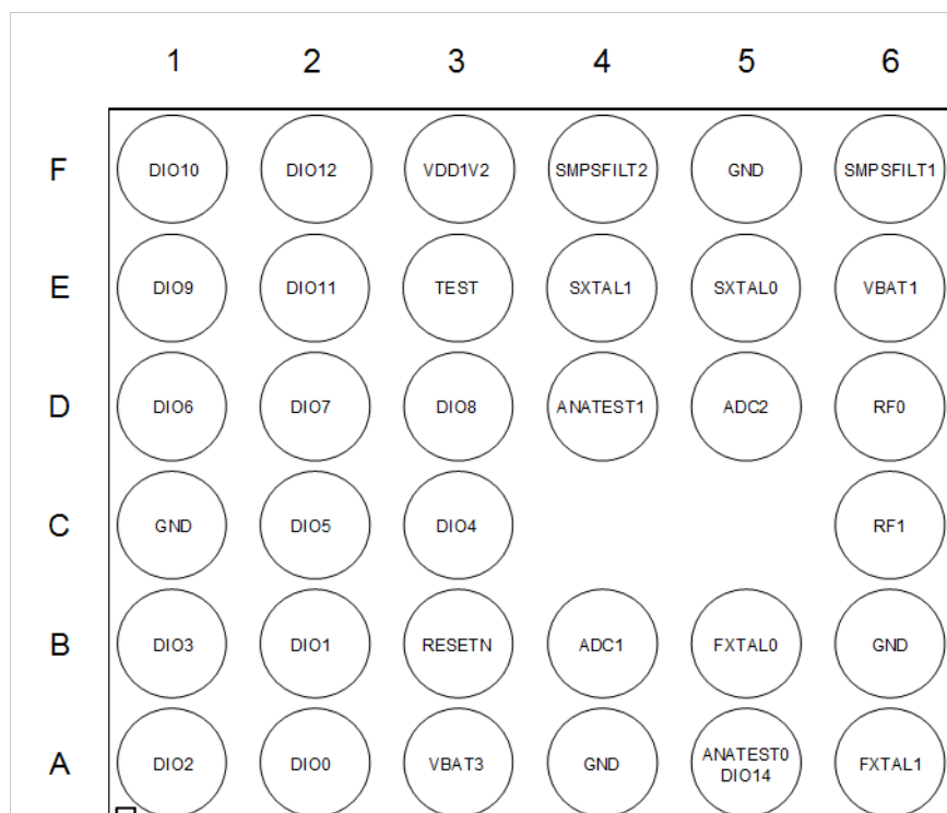
Figure 23. BlueNRG-1 ball out bottom view (WLCSP34)
