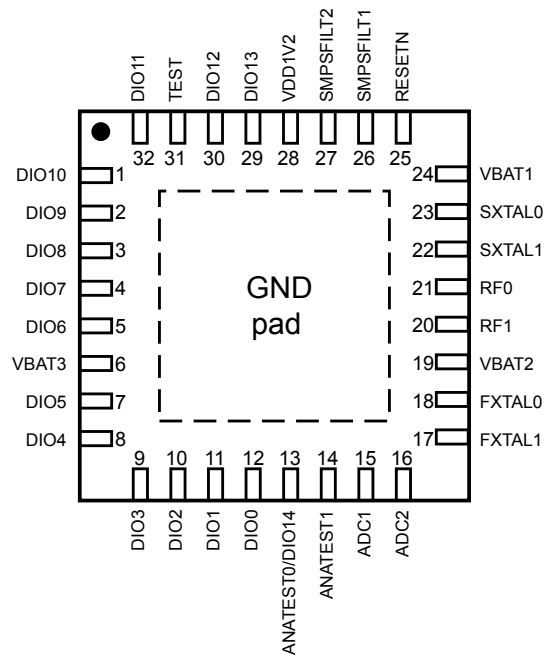
Figure 21. BlueNRG-1 pinout top view (VFQFPN32)
