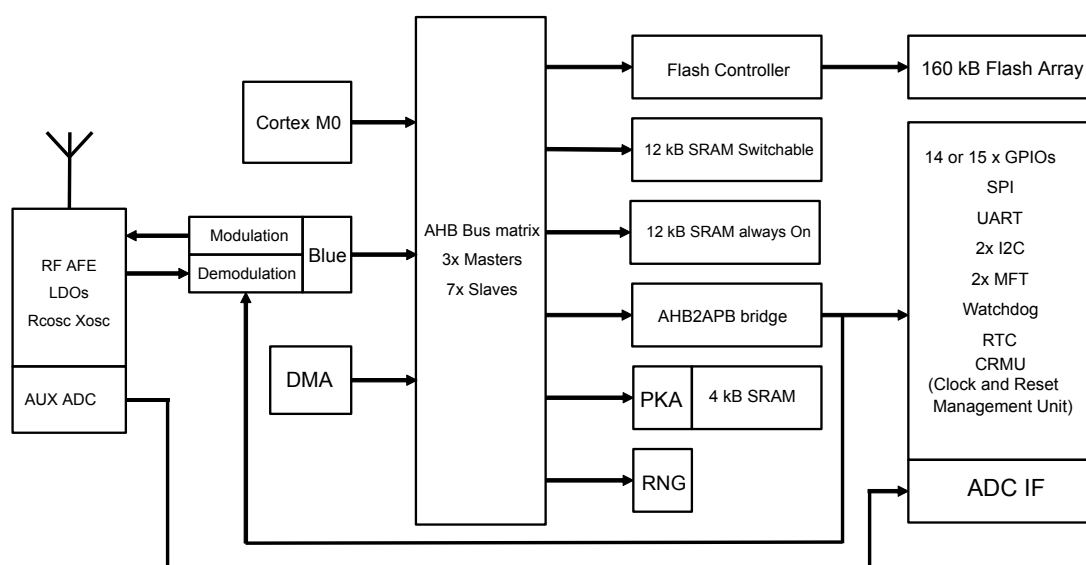
Figure 1. BlueNRG-1 architecture
