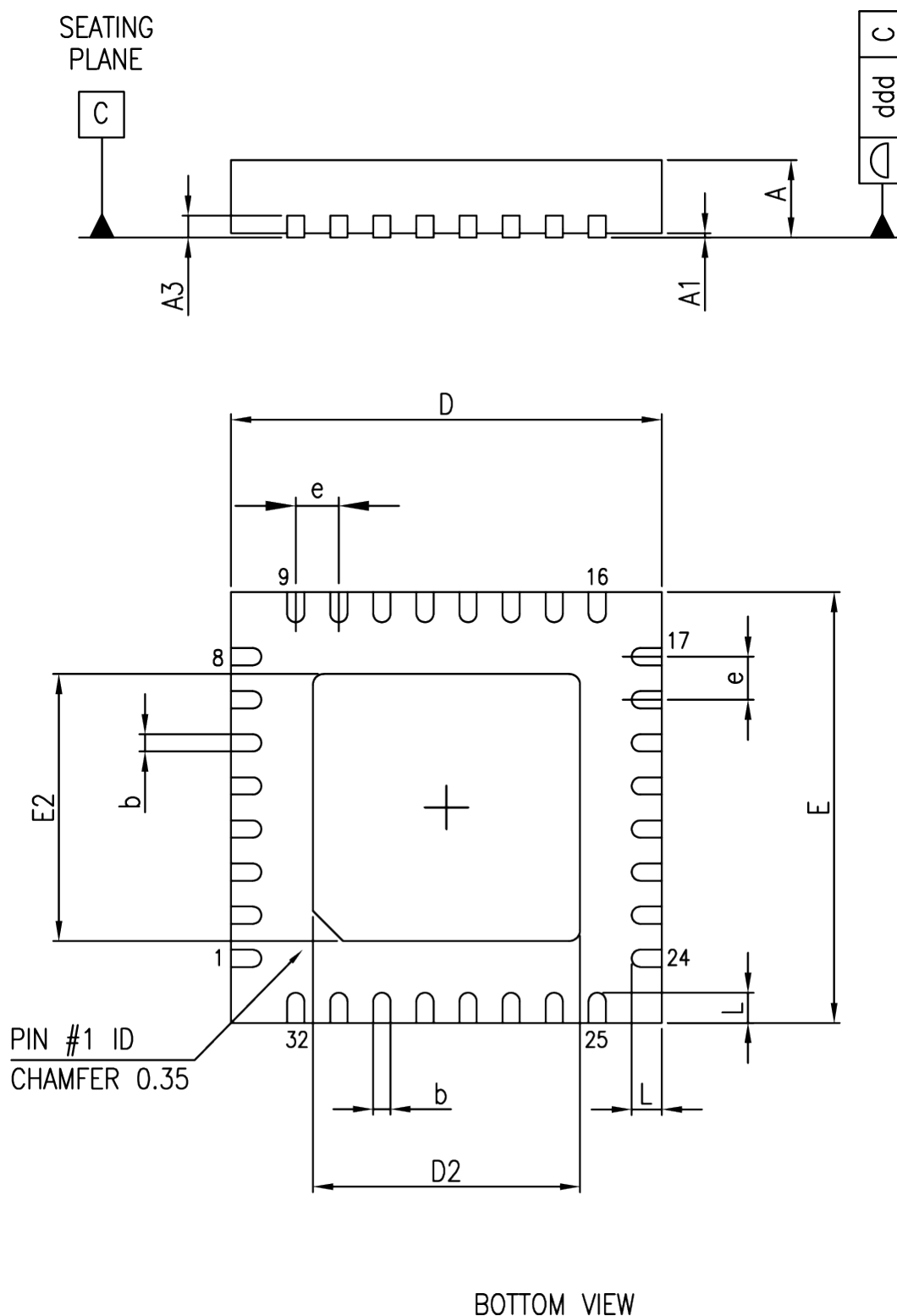
Figure 35. VFQFPN32 (5 x 5 x 1 pitch, 0.5 mm) package outline (BlueNRG-132S)
