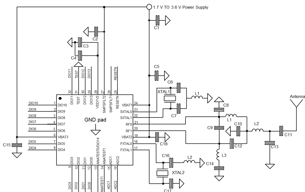
Figure 25. Application circuit: nonactive DC-DC converter VFQFPN32 package
