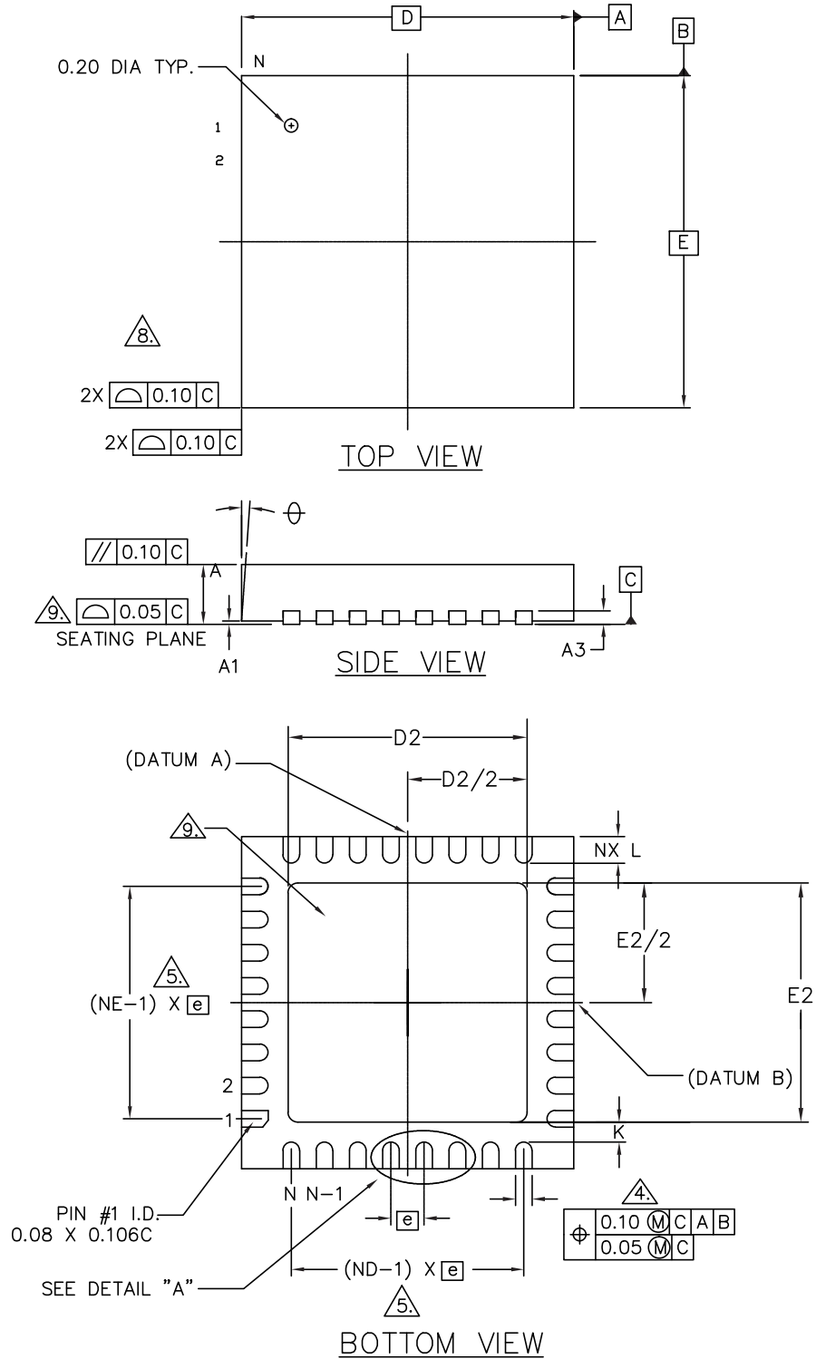
Figure 33. VFQFPN32 (5 x 5 x 1 pitch 0.5 mm) package outline (BlueNRG-132)
