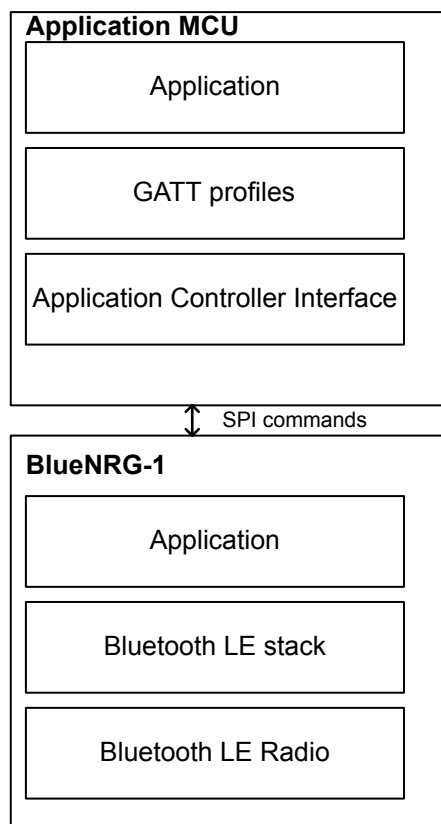
Figure 4. BlueNRG-1 network processor RF software layers
