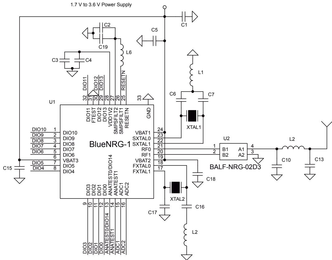
Figure 28. Application circuit: active DC-DC converter VFQFPN32 package with BALF-NRG-02D3 balun
