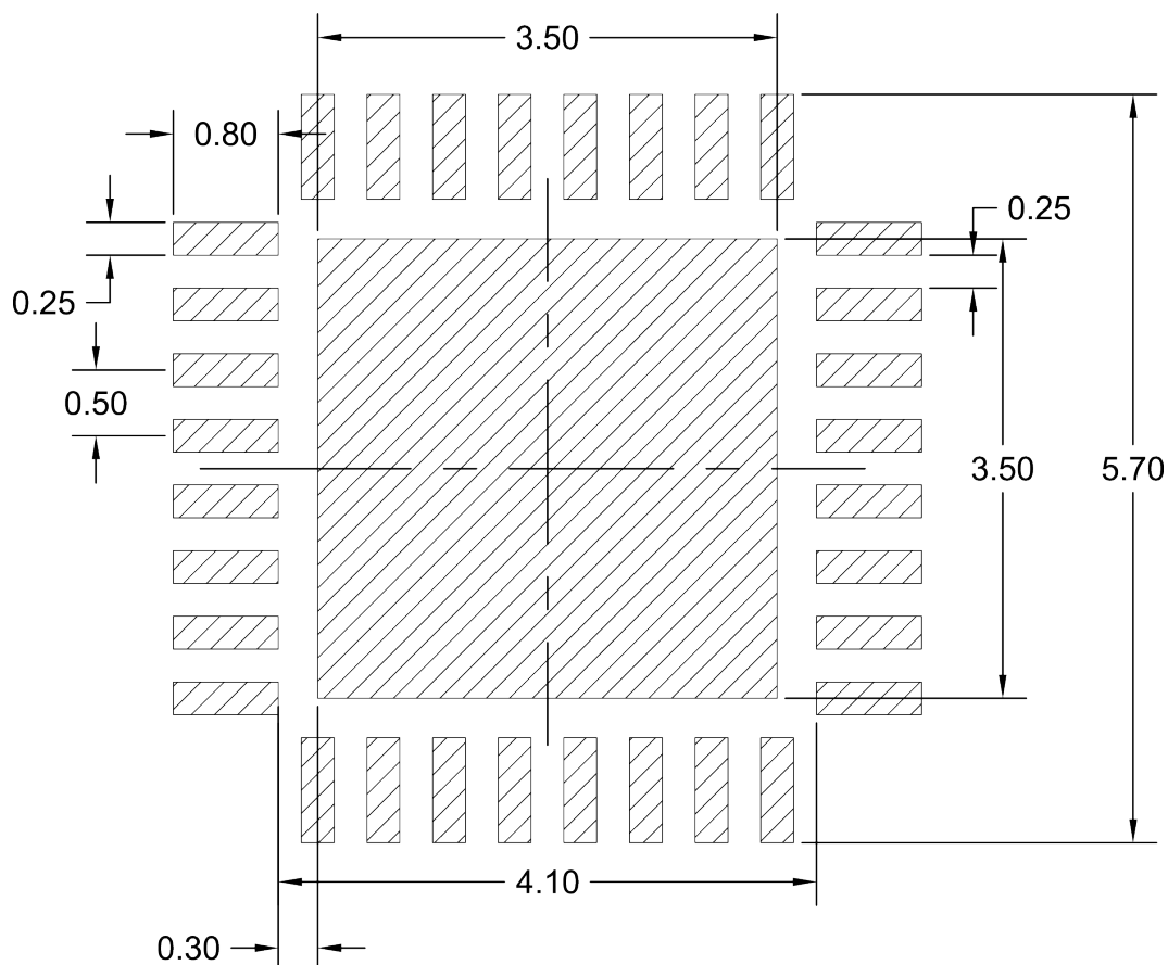
Figure 36. Footprint example - VFQFPN32 (BlueNRG-132S)
