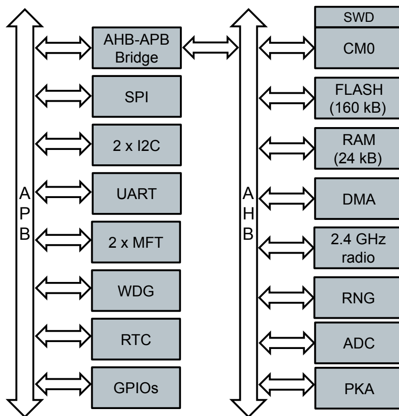
Figure 2. BlueNRG-1 bus architecture
