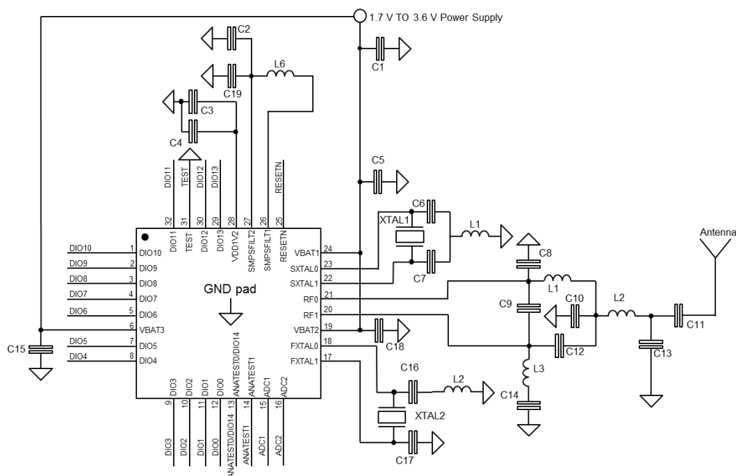
Figure 24. Application circuit: active DC-DC converter VFQFPN32 package
