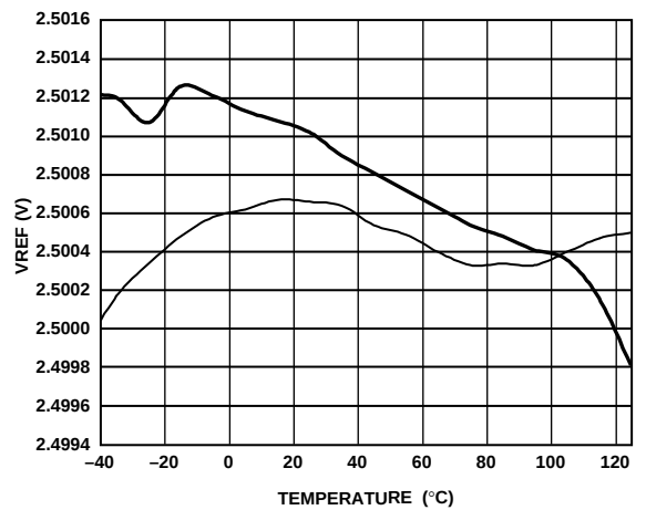
Figure 21. Typical Reference Voltage Output vs. Temperature (2 Units)
