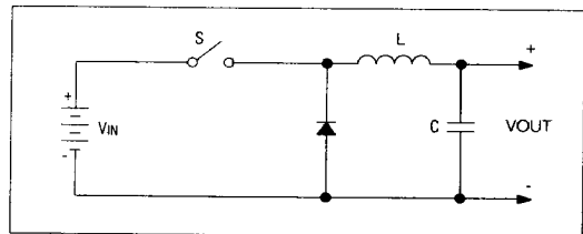
Figure 1. Simplified Step-Down Converter
