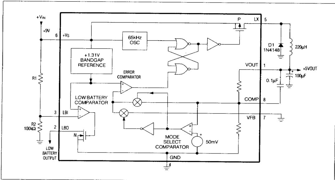
Figure 2. MAX638 Block Diagram and Typical Circuit
