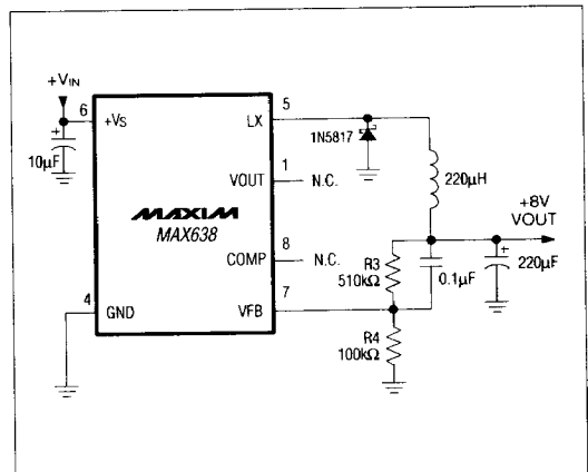
Figure 4. Adjustable Output Operation
