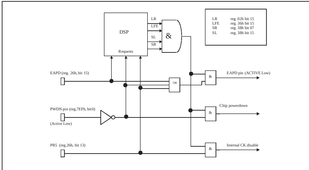
Figure 7. Powerdown management
