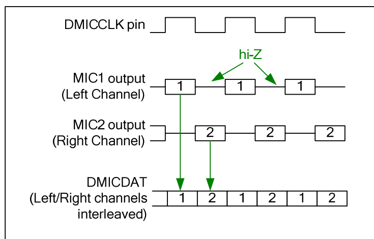
Figure 28 Digital Microphone Interface Timing
