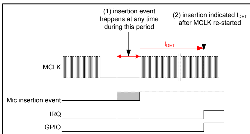
Figure 25 MICBIAS Detection events without MCLK
