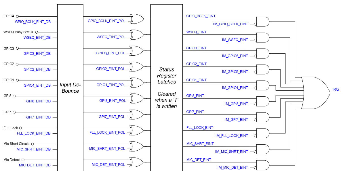
Figure 60 Interrupt Controller
