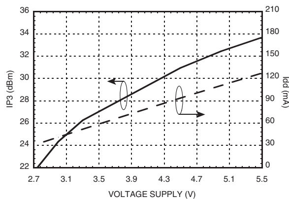
Output IP3 and Idd vs. Supply Voltage @ 1700 MHz
