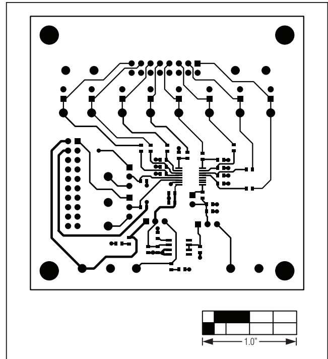
Figure 26. MAX11614 EV Kit Daughter Board PCB Layout—Top
