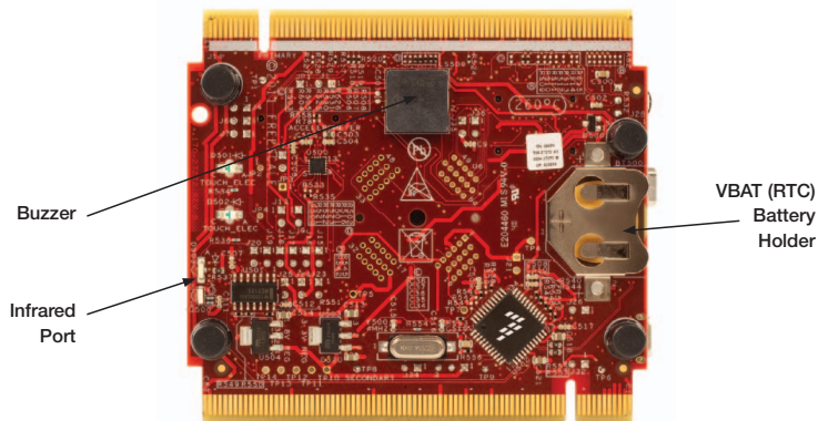
Figure 2: Back side of TWR-K20D50M module.
