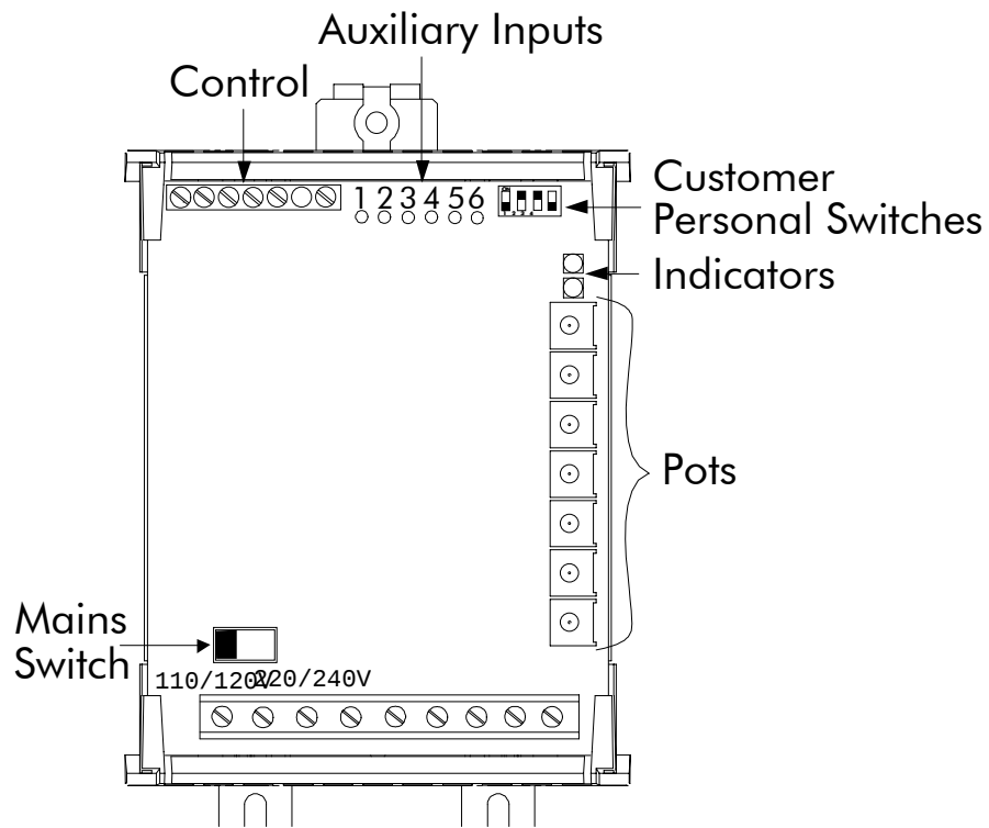
Figure 2.1 Recognition Drawing
