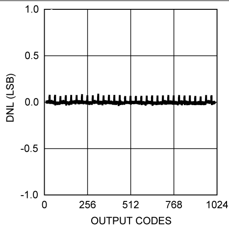
Figure 5. DNL at V_A = 5 V
