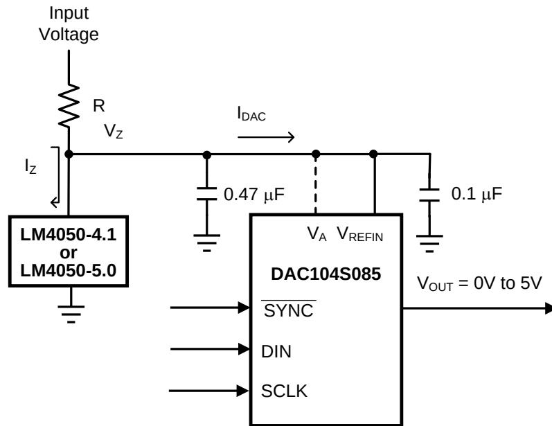
Figure 36. The LM4050 as a Power Supply
