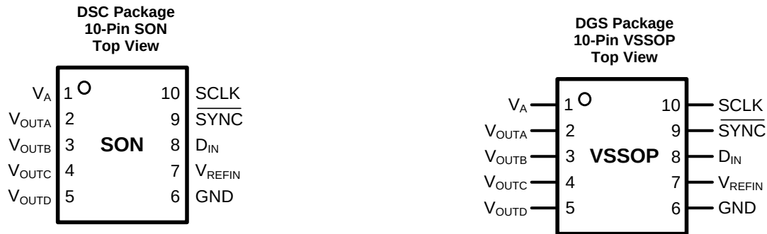
Pin Functions
