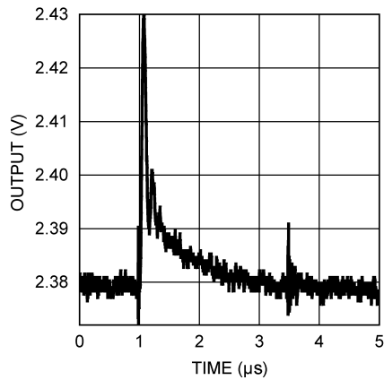
Figure 37. 5-V Glitch Response
