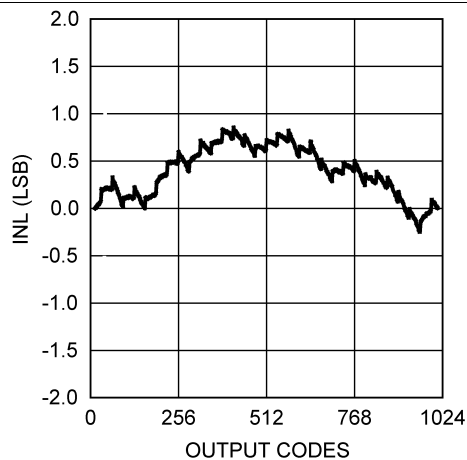
Figure 3. INL at V_A = 5 V
