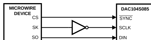
Figure 32. Microwire Interface
