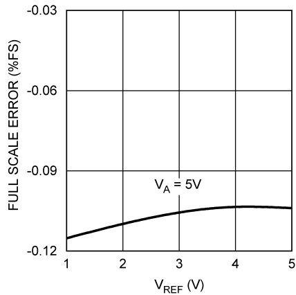
Figure 20. Full-Scale Error vs V_{REF}
