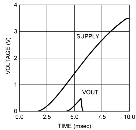
Figure 38. Power-On Reset
