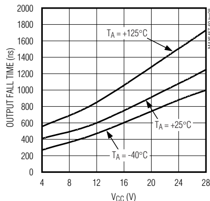
OUTPUT FALL TIME vs. SUPPLY VOLTAGE
