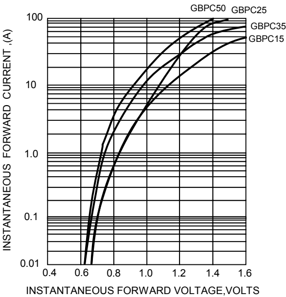
FIG.3-TYPICAL FORWARD CHARACTERISTICS
