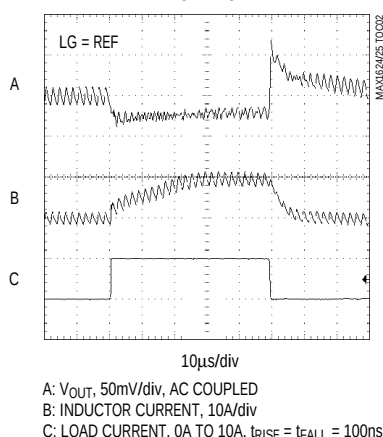
MAX1624 LOAD-TRANSIENT RESPONSE (WITH GLITCHCATCHER) (1.1V)
