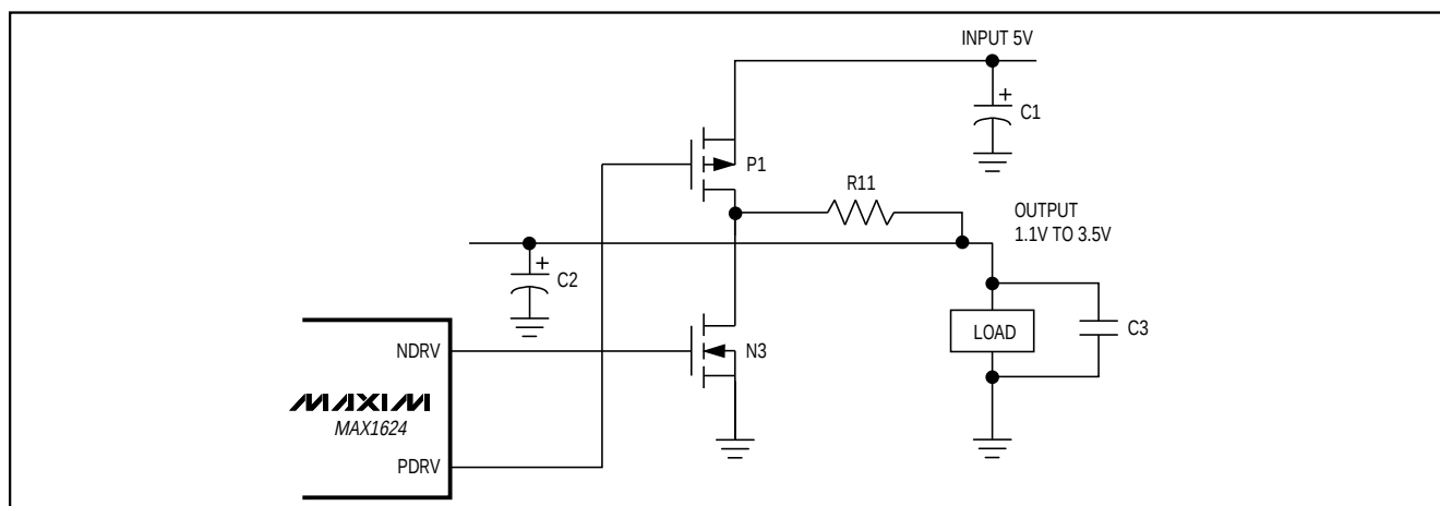
Figure 10. GlitchCatcher Circuit
