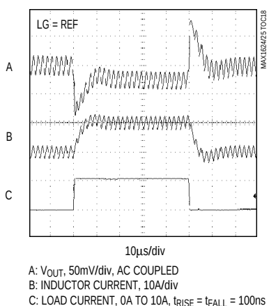
MAX1624 LOAD-TRANSIENT RESPONSE (WITHOUT GLITCHCATCHER) (2.5V)
