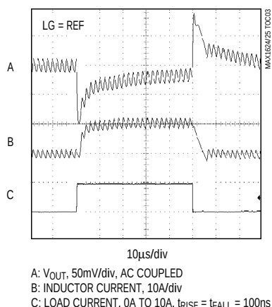
MAX1624 LOAD-TRANSIENT RESPONSE (WITHOUT GLITCHCATCHER) (1.1V)
