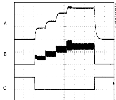
MAX1624 STARTUP AND STANDBY RESPONSE
