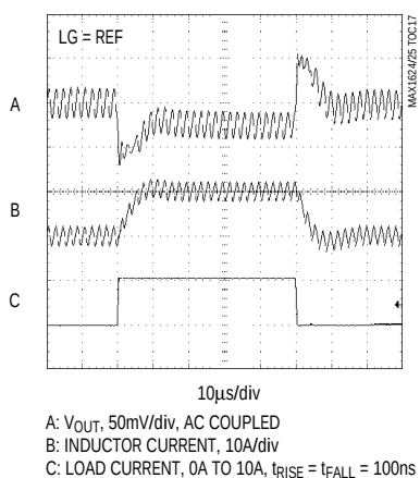
MAX1624 LOAD-TRANSIENT RESPONSE (WITH GLITCHCATCHER) (2.5V)
