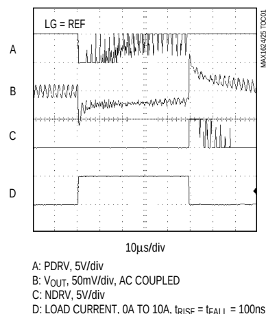
MAX1624 LOAD-TRANSIENT RESPONSE DETAIL (WITH GLITCHCATCHER) (1.1V)
