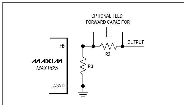
Figure 9. MAX1625 Optional Feed-Forward Compensation Capacitors
