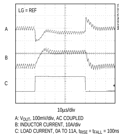
MAX1624 LOAD-TRANSIENT RESPONSE (WITHOUT GLITCHCATCHER) (3.5V)
