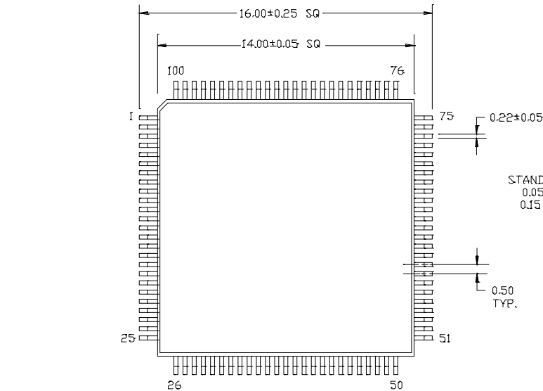
100-Lead Lead (Pb)-Free Thin Plastic Quad Flat Pack (TQFP) A100
