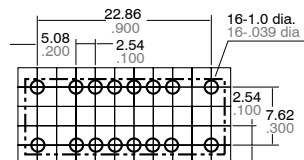
PC board pattern (Copper-side view)
