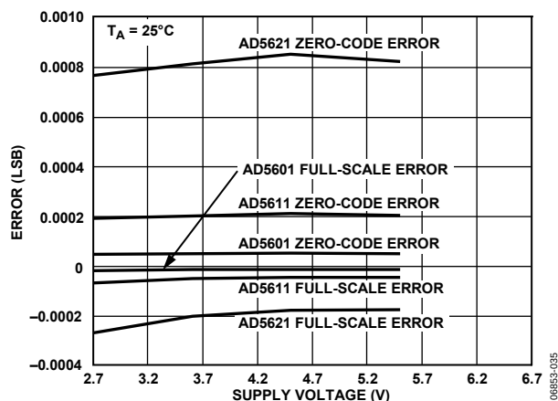
Figure 36. Zero-Code Error and Full-Scale Error vs. Supply Voltage at 25^\circ\text{C}
