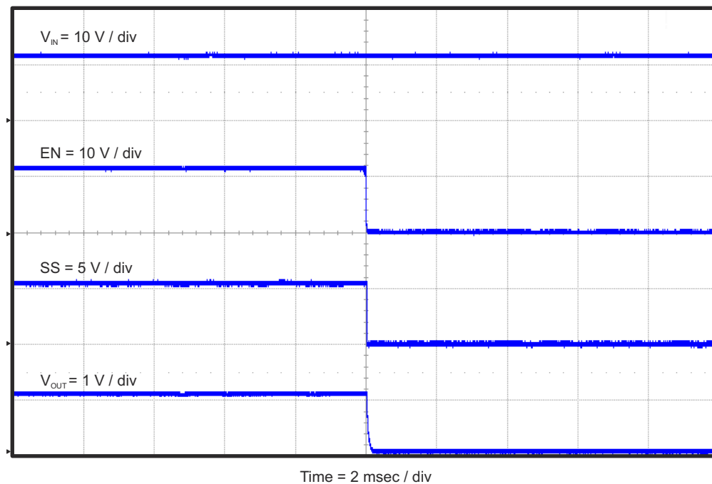
Figure 4-13. TPS54239EEVM-056 Shut-Down Relative to EN with SS
