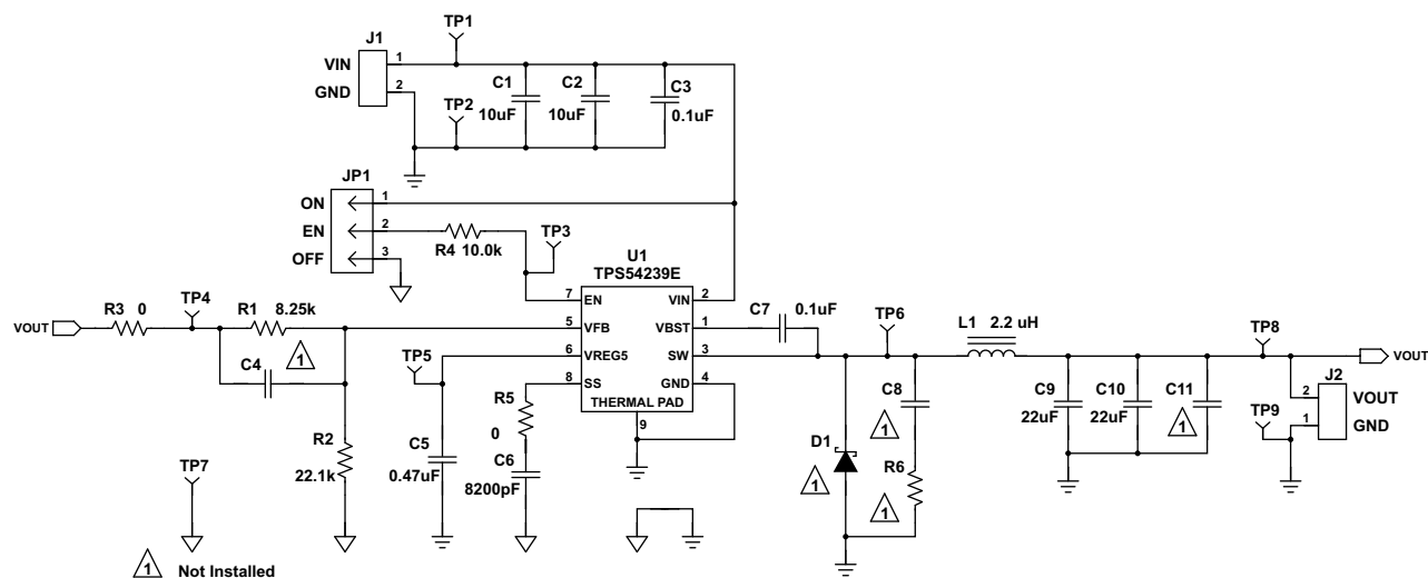
Figure 6-1. TPS54239EEVM-056 Schematic Diagram
