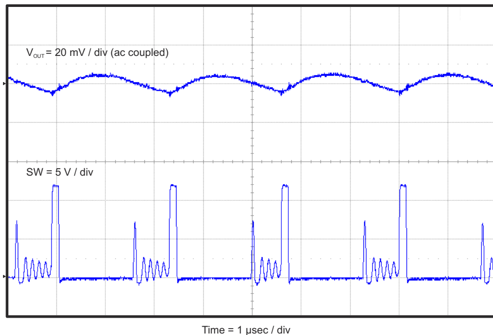
Figure 4-7. TPS54239EEVM-056 Output Voltage Ripple ( I_{OUT} = 50 \text{ mA} )
