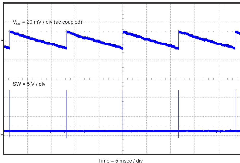
Figure 4-8. TPS54239EEVM-056 Output Voltage Ripple ( I_{OUT} = 0 \text{ A} )
