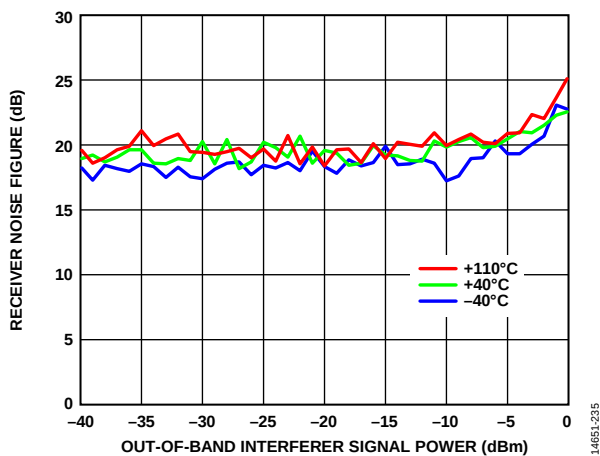
Figure 196. Receiver Noise Figure vs. Out-of-Band Interferer Signal Power, 5400 MHz LO, 5600 MHz CW Interferer, NF Integrated over 7 MHz to 10 MHz
