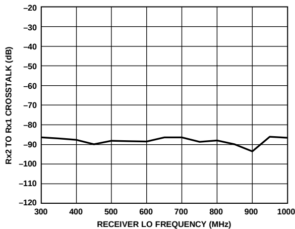
Figure 18. Rx2 to Rx1 Crosstalk vs. Receiver LO Frequency, 100 MHz RF Bandwidth, CW Tone 3 MHz Offset from LO
