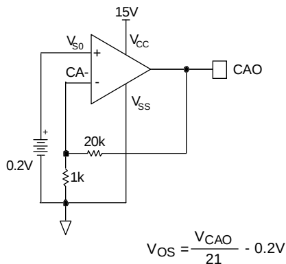
Figure 8. Operational Amplifier Input Offset Voltage Measurement
