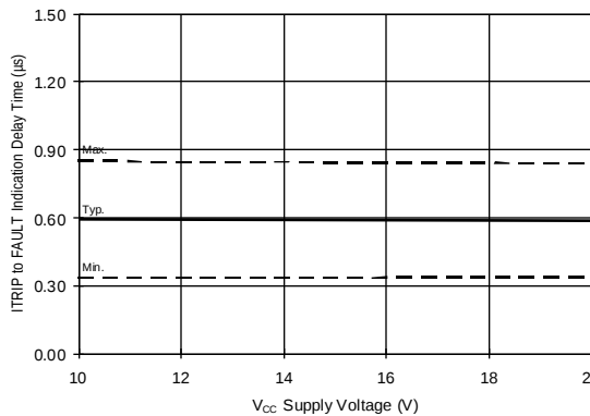
Figure 16B. ITRIP to \overline{\text{FAULT}} Indication Time vs. Voltage
