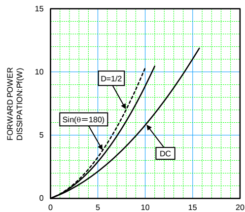
AVERAGE RECTIFIED FORWARD CURRENT: I_o (A) I_o - P CHARACTERISTICS
