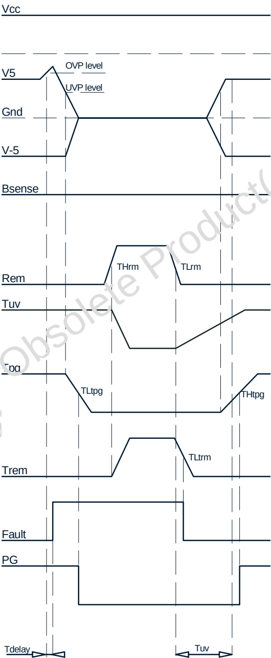
Figure 5: OVP Function Rem On/Off, Tuv start up
