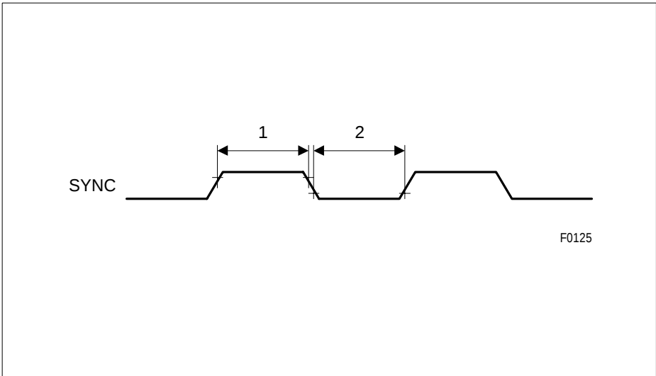
Figure 99 SYNC Timing
