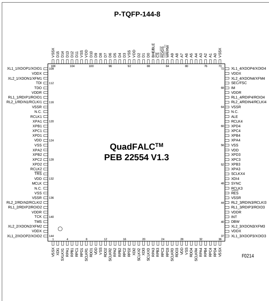
Figure 4 Pin Configuration
