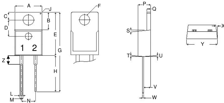
Package TO-220-2
