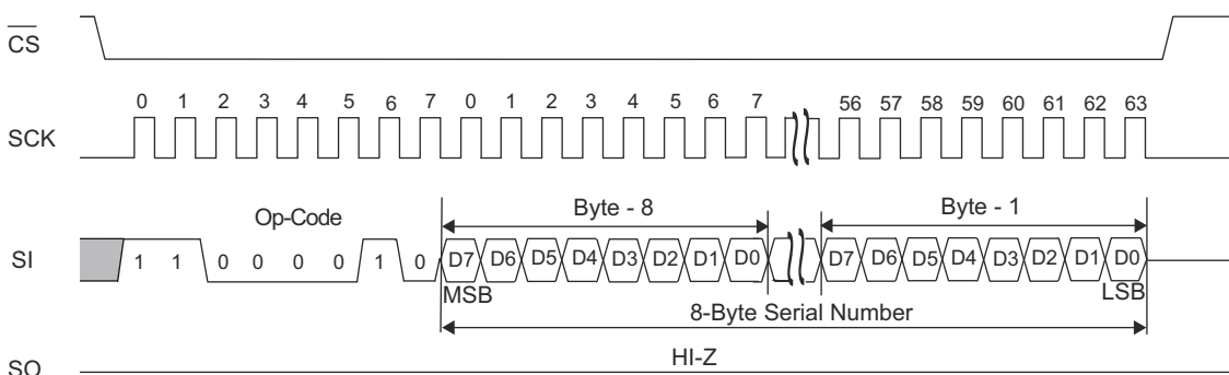
Figure 22. WRSN Instruction
