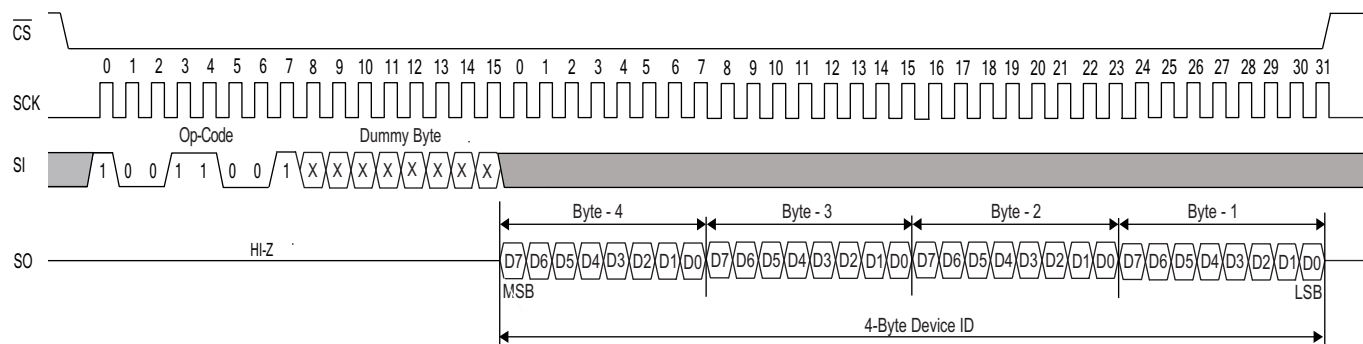
Figure 26. FAST_RDID instruction
