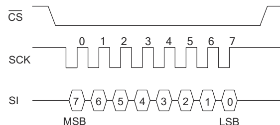
Figure 6. SPI Mode 3
