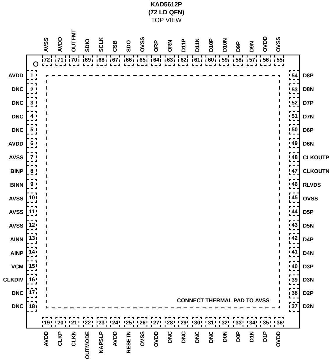
FIGURE 3. PIN CONFIGURATION
