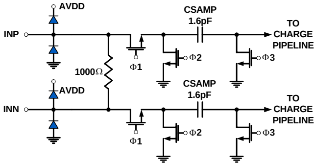
FIGURE 42. ANALOG INPUTS
