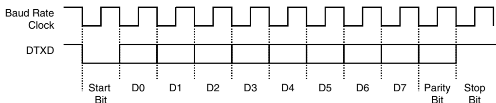
Figure 26-10. Character Transmission
