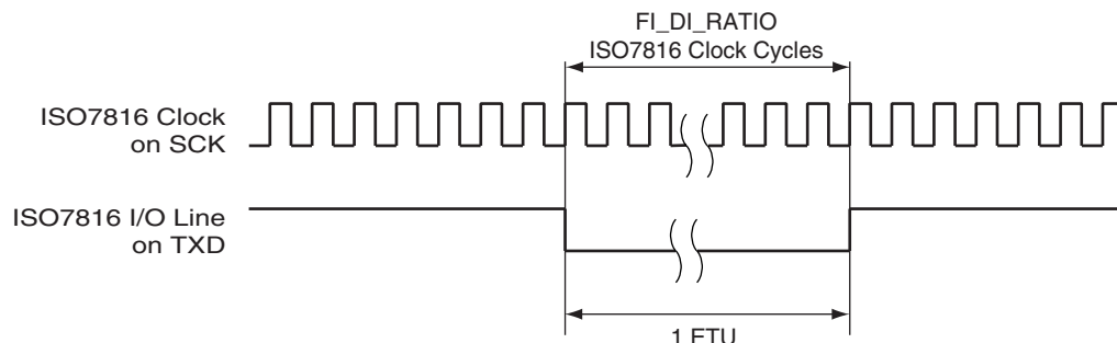
Figure 30-4. Elementary Time Unit (ETU)
