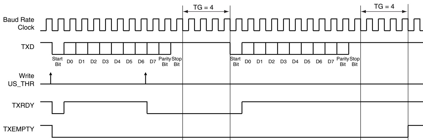
Figure 30-12. Timeguard Operations
