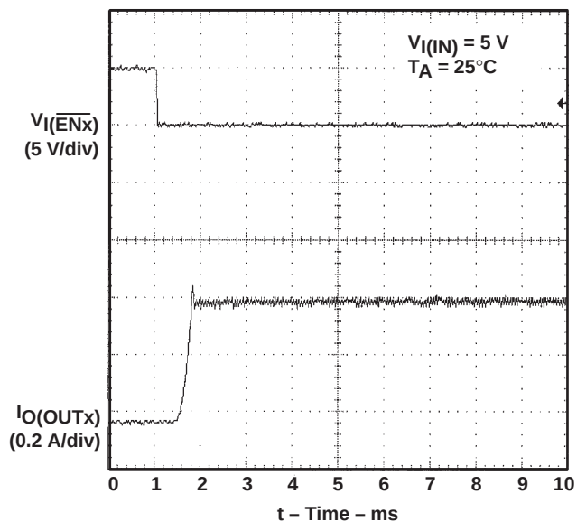
Figure 6. TPS2046, Short-Circuit Current, Device Enabled into Short
