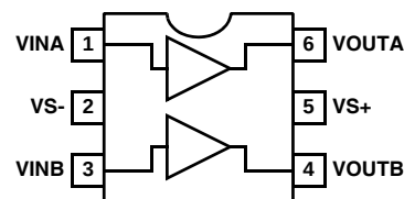
EL5221 (6 LD SOT-23) TOP VIEW
