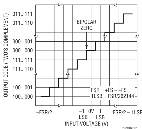
Figure 2. LTC2379-18 Transfer Function
