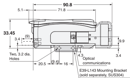
Mounting Holes
