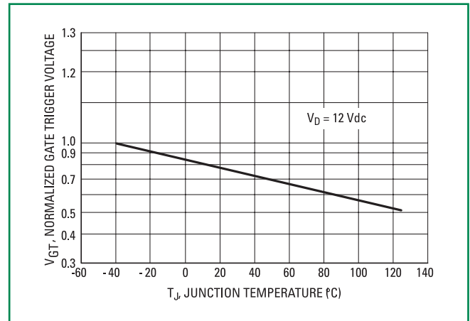
Figure 4. Typical Gate Trigger Voltage vs Temperature
