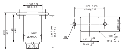
SUGGESTED MOUNTING CUTOUT
