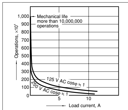
Life curve
