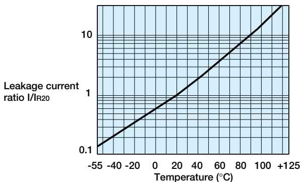
LEAKAGE CURRENT vs. TEMPERATURE
