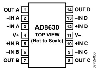
Figure 4. 14-Lead SOIC_N (R-14) and 14-Lead TSSOP (RU-14)
