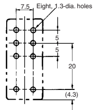
Mounting Holes
