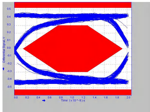
Figure 8-17. High-Speed Downstream Port 2
