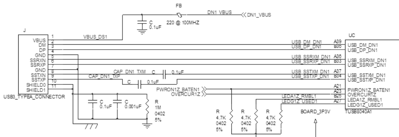
Figure 8-4. Downstream Port 2 Implementation
