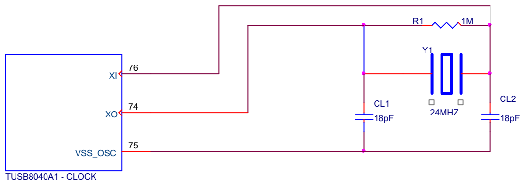
Figure 6-1. TUSB8040A1 Clock
