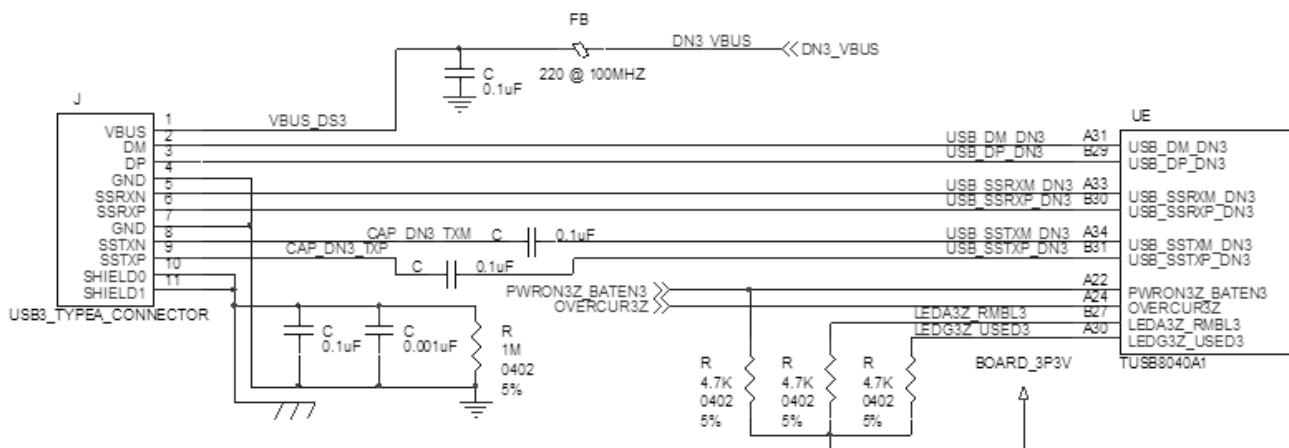
Figure 8-6. Downstream Port 4 Implementation
