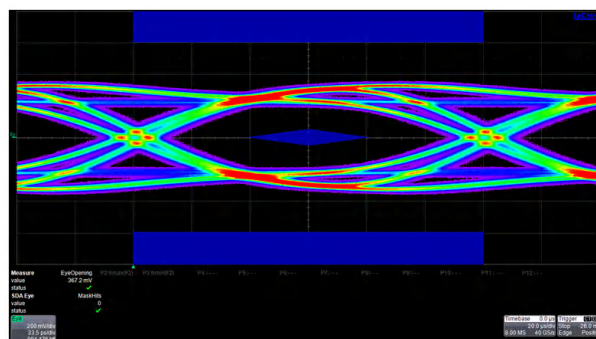
Figure 8-11. Downstream Port 1
