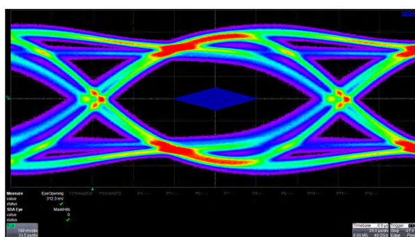
Figure 8-13. Downstream Port 3
