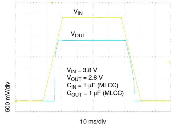
Figure 43. Turn-on/off – Slow Rising V_{IN} - I_{OUT} = 300 mA
