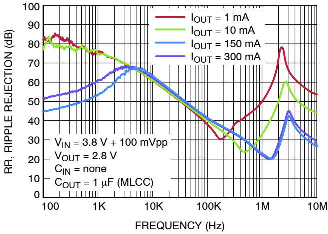
Figure 26. Power Supply Rejection Ratio, V_{OUT} = 2.8 V
