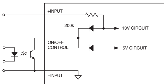
Figure 2. Driving the Positive Polarity On/Off Control Pin
