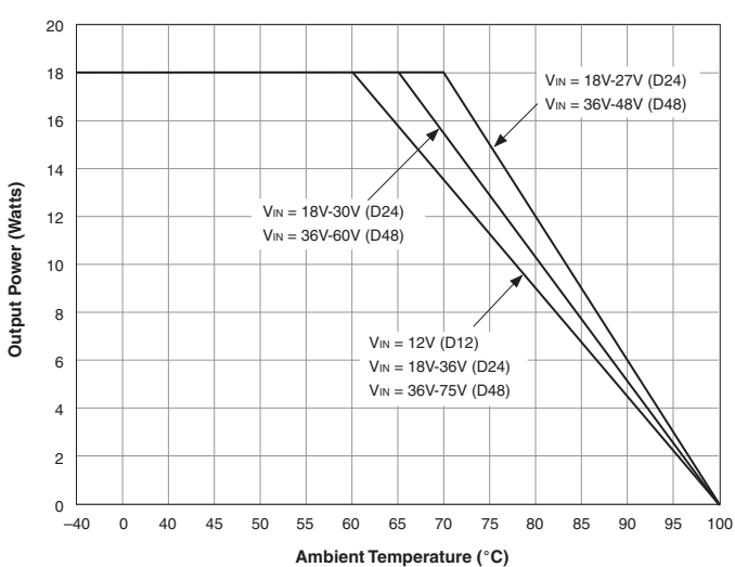
Temperature Derating Curves for 15V Output Models
