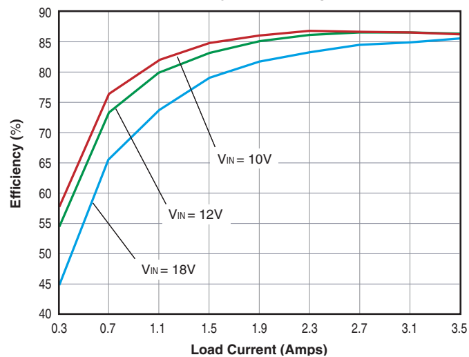
UEP-5/3500-D12 Efficiency vs. Line Voltage and Load Current
